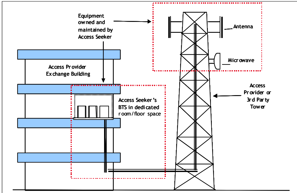
Tower Space with Outdoor Cabin/Equipment Configuration
