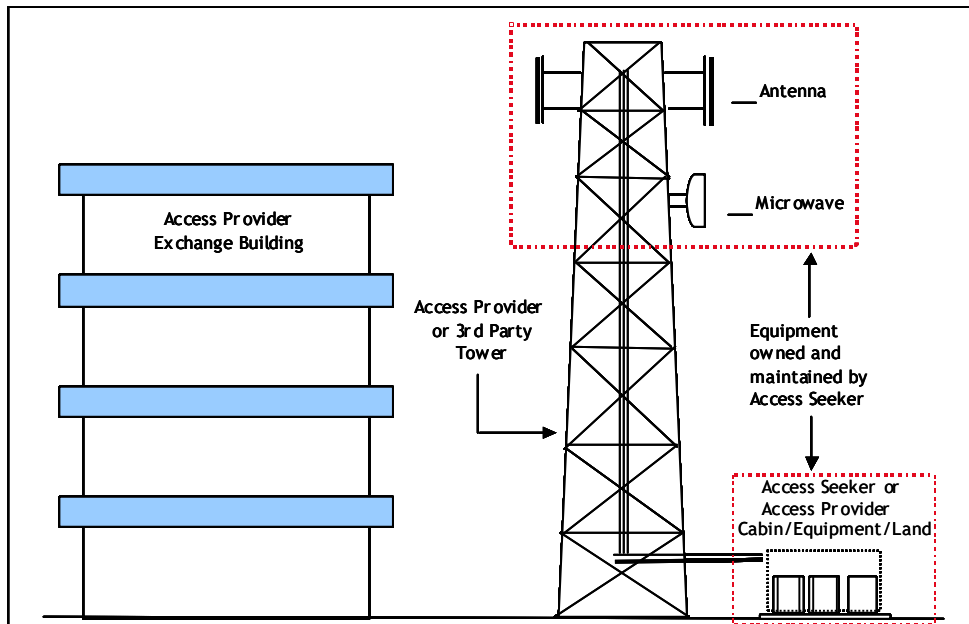
Tower Space with Indoor Cabin/Equipment Configuration
